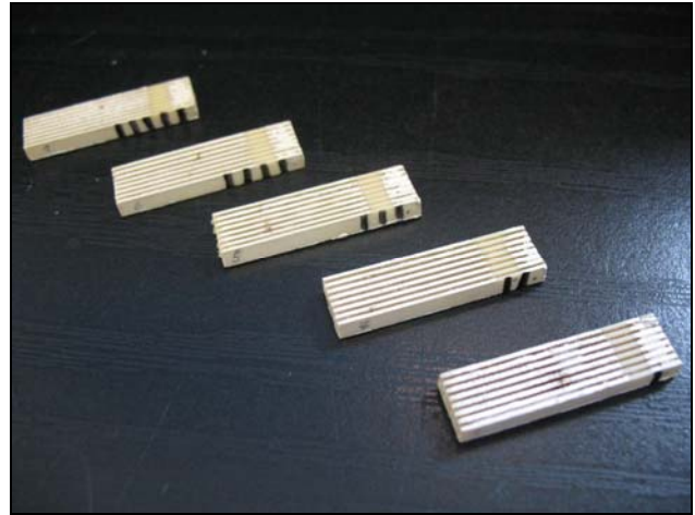
Figure 2.2 Piezo-composite samples used for the tests.
