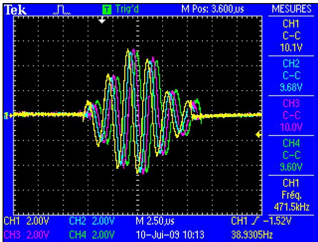
Figure 5.1 Four excitation signals to obtain selective emission.
