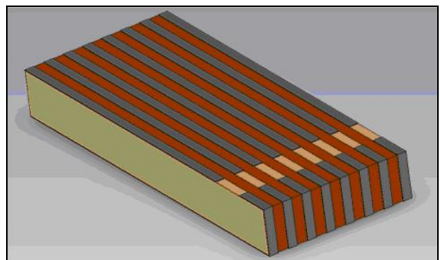
Figure 1.1 Schematic view of a piezo-composite patch featuring 8 elements.
