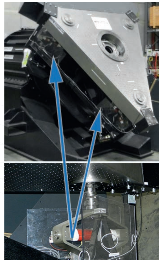
Fig. 3: APA500XXL integrated in the Tip Tilt platform of the M5 field Stabilization unit
