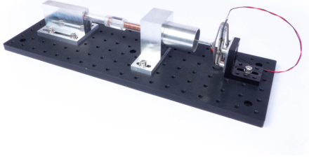
Fig. 9 : Piezo pulse tube stirling refrigerator (demo kit)
