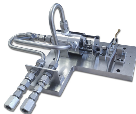
Fig. 3 : 200 Bar high pressure regulation valve
