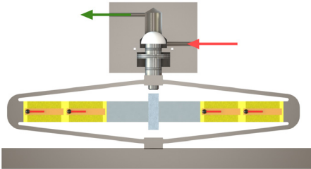
Fig. 1 : Piezo regulation valves principle
