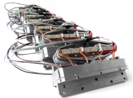
Fig. 8 : Batch of ASPIC SJA mechanisms
