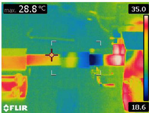
Fig. 10 : Thermal imaging of the pulse tube heat pumping process
