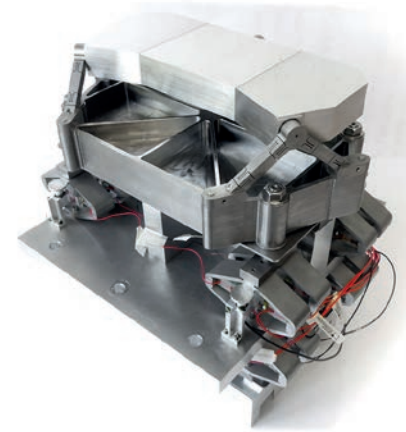
View of MEFISTO mechanism
