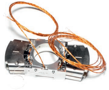
Fig. 1: Space Voice Coil 1 for MTG Scanning Assembly for SENER
