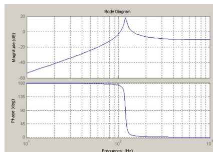
Frequency response of a actuator in proof mass configuration.
