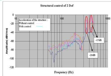
Performance and frequency response of the Active Mass Damper.
