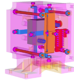
Mechanical view of the PM900M based on a APA900M piezoelectric actuator.
