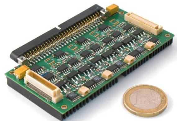
Fig. 2: 4-channel fully featured (pulse-echo) SHM embedded platform
